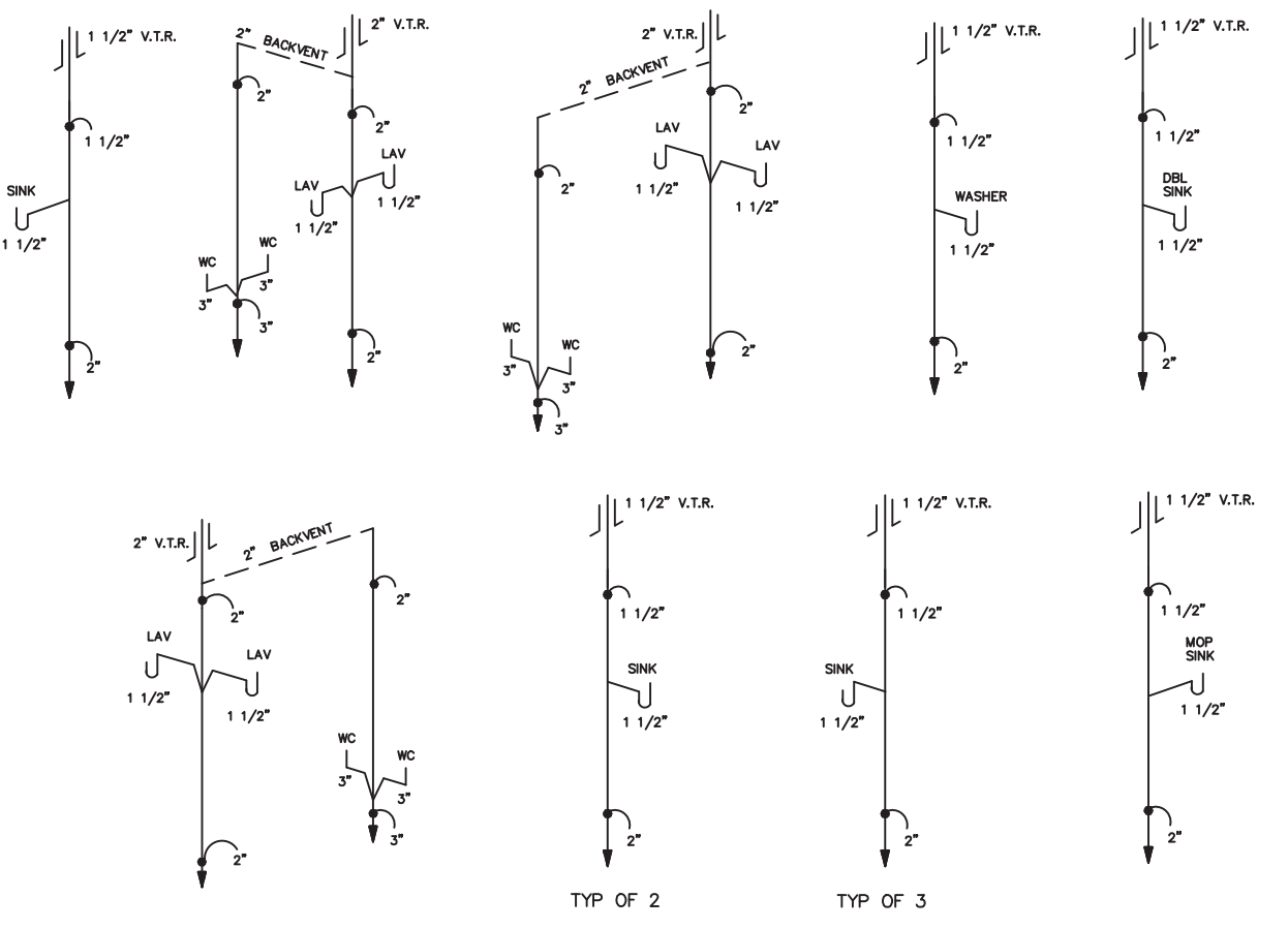
DWV RISER NTS
