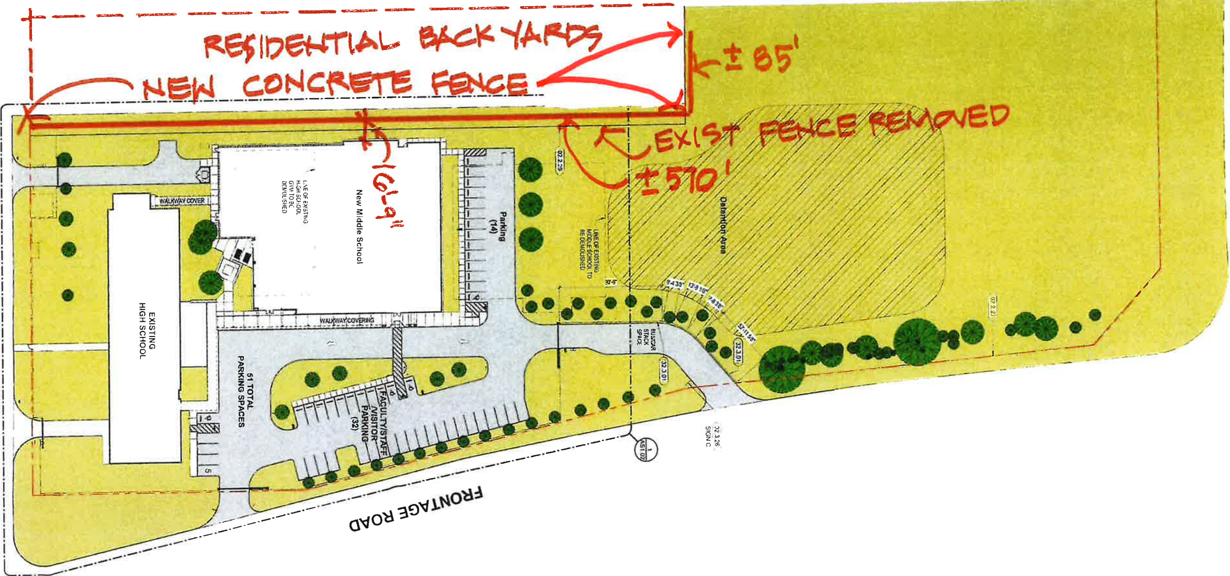
VILLAGROVE DRIVE OVERALL SITE PLAN - BASE BID 1" = 40'-0"
